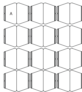
#811 12" Retaining Wall Pieces per layer: 24 Layers per pallet: 6
